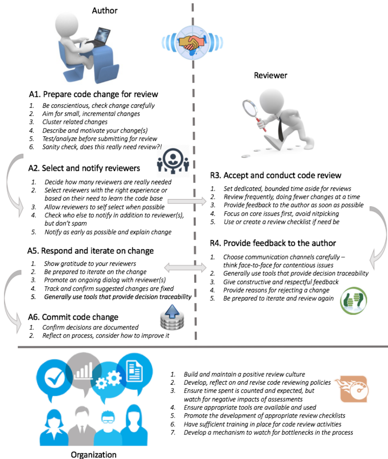
Figure 2: An overview of the best practices we suggest for authors of code changes, reviewers of changes, and organizations. The diagram also shows the main steps of the code review life cycle.
